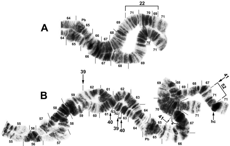
Figure 4. Chromosome arm III L of male larvae of Simulium bergi . A Distal half of chromosome, showing heterozygous expression of the common Y-linked inversion III L-22 B Complex sex-chromosome configuration, showing one homologue with III L-39,40 and the other with III L-41,52+hc71+7 extra bands; hc = heterochromatic block, Pb = parabalbiani, * = 7 additional bands inserted in one homologue.
