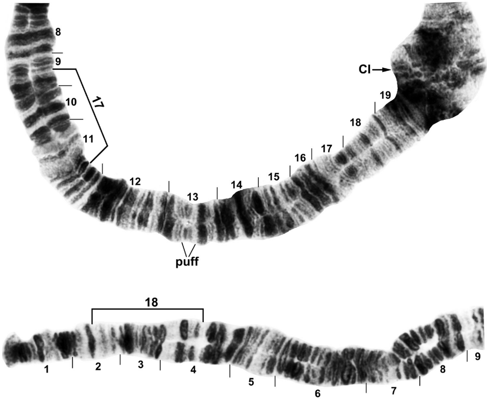
Figure 1. Chromosome arm IS of Simulium bergi (male larva), representing the Simulium subgeneric standard. Limits of two autosomal inversions and a puff are indicated with brackets on the standard sequence. CI = centromere of chromosome I.
