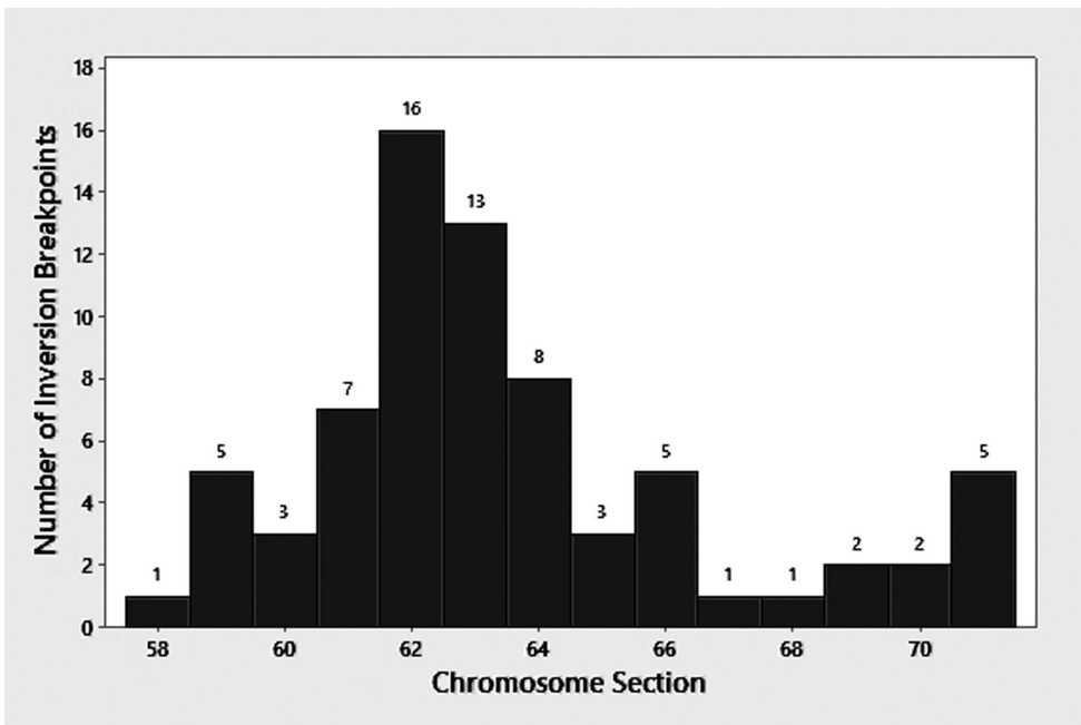
Figure 5. Distribution of breakpoints of 36 sex-linked inversions in the IIL arm of Simulium bergi . Breakpoints are plotted according to section number of the standard banding sequence for the subgenus Simulium . Breakpoints falling at the junction of two sections are tallied for the distalmost of the two sections.
