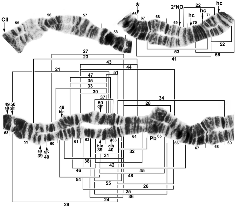
Figure 2. Composite map of chromosome arm IIL of Simulium bergi (female larva), representing the Simulium subgeneric standard. Breakpoints of sex-linked inversions are indicated with brackets or arrows. Ordering the two independent sets of chromosome fragments indicated by the letters “a” through “h” will produce the inverted sequence for IIL-39,40 and IIL-49,50. CII = centromere of chromosome II, hc = insertion point for heterochromatic block, Pb = parabalbiani, 2°NO = location of secondary nucleolar organizer, * = insertion point for 7 additional bands (only when IIL-41 is present).
