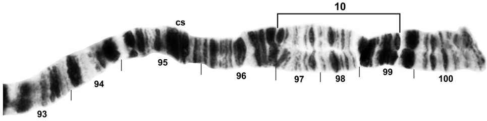
Figure 3. Distal half of chromosome III L of Simulium bergi (female larva), representing the Simulium subgeneric standard. Limits of autosomal inversion III L-10 are indicated with a bracket on the standard sequence; cs = cup and saucer marker.
